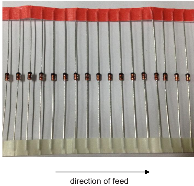
Fig 2. Product orientation in carrier tape
